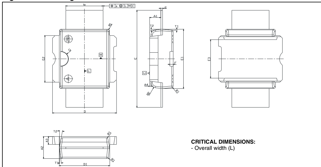
Figure 6. Package dimensions
